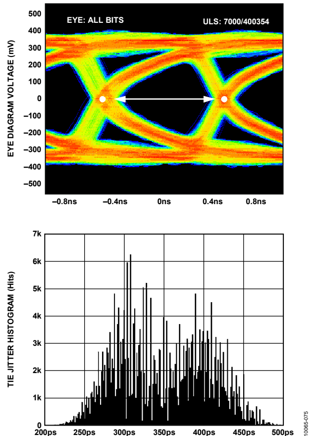
Figure 72. Data Eye for LVDS Outputs in ANSI-644 Mode with Trace Lengths Less than 24 Inches on Standard FR-4 Material, External 100 Ω Far-End Termination Only
